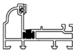
44MM ALUMINIUM THRESHOLD (OVOLO)
